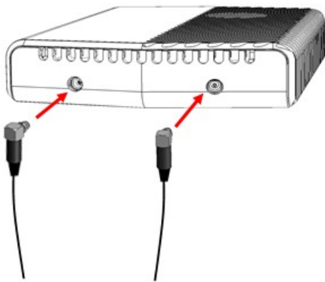
Connecting the Antennas to the Air Unit
