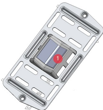
Connecting the Mounting Plate to a Bar on the Drone
