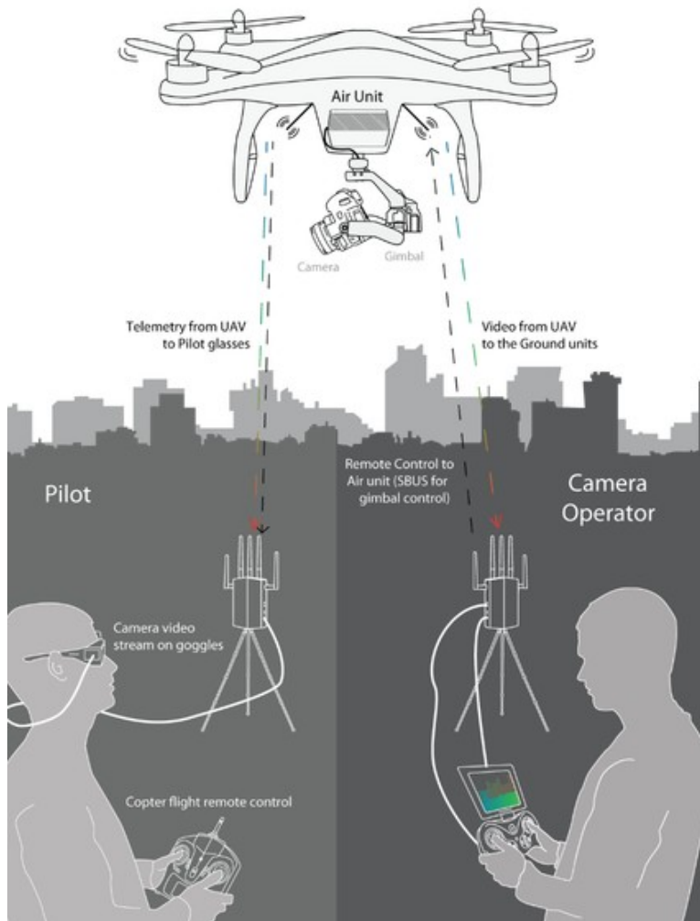
How CONNEX Works
