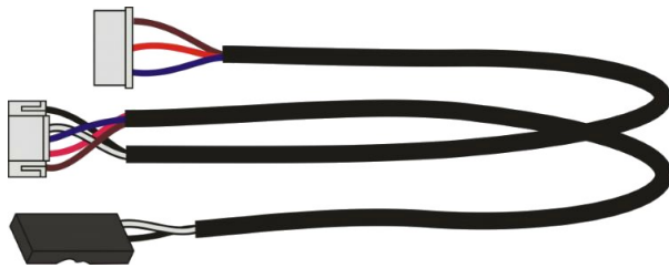
Air Unit MAVLink Telemetry and S.BUS cable
